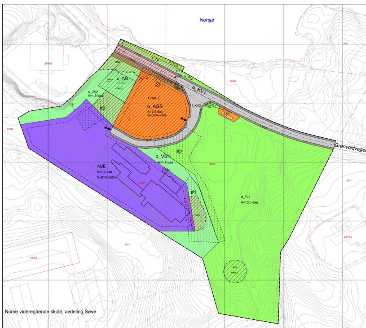
Figur 4-1: Plankart
